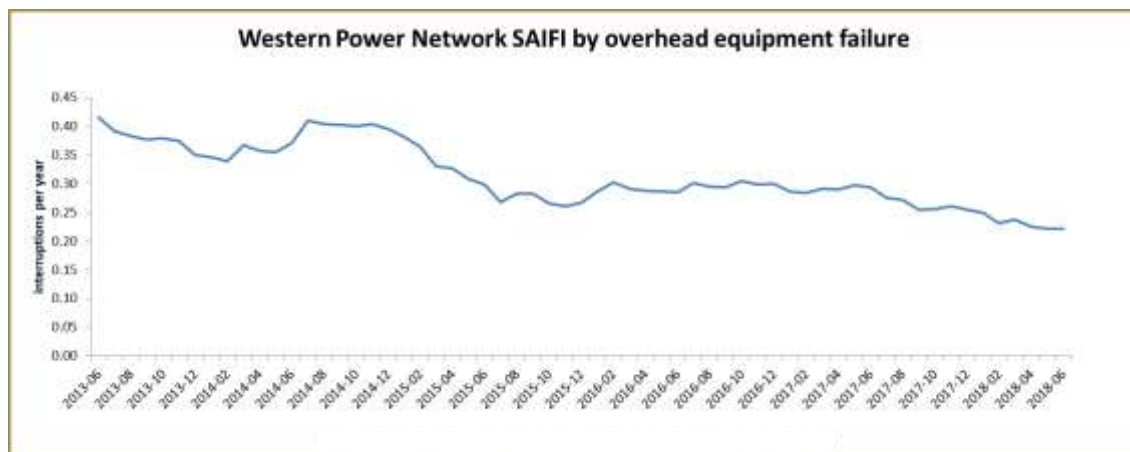
Figure B.1: Western Power Network SAIFI – overhead equipment failure cause trend
