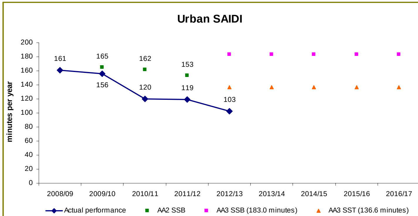
Figure 5: Urban SAIDI
