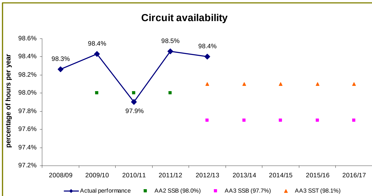
Figure 13: Circuit availability
